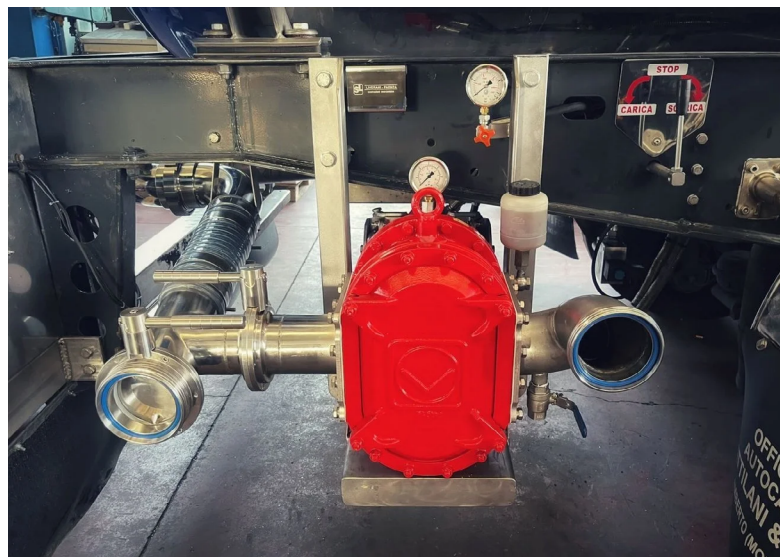
Vogelsang rotationspumpe VX136-140Q med Automatic Supply Unit (ASU)
