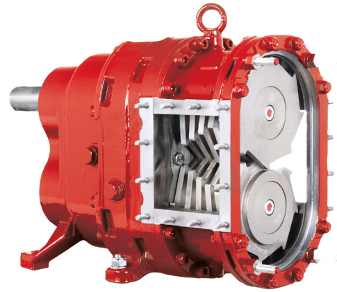
Vogelsang wastewater grinder XRipper
