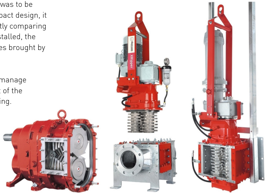
Twin-shaft grinder for sewer and WWTP
