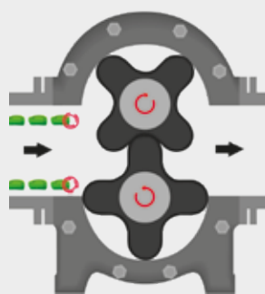
Rotationspumpe i konventionel version
