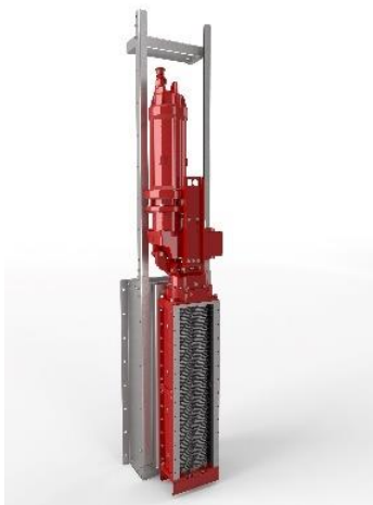
Image 3: Extra narrow X Ripper XRC100 with Sewer Integration Kit (SIK) for narrow channels.
