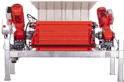
Image 1: The industrial grinder RedUnit XRL260 ensures high throughput rates.
